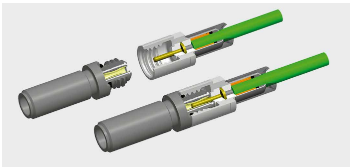
KIAG 10-32 pos. int. - connector with integrated thread
