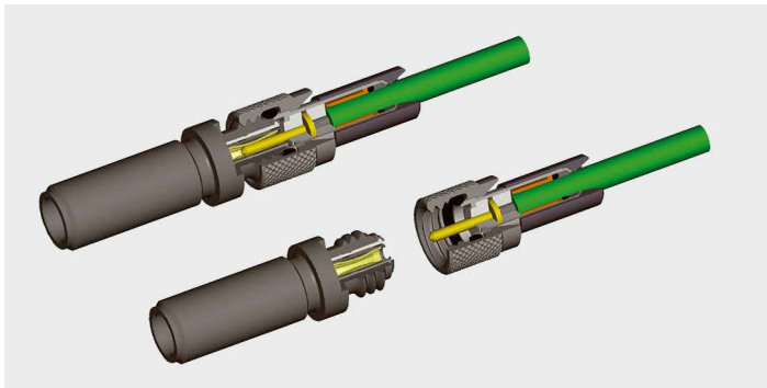
KIAG 10-32 pos. – connector with rotatable swivel nut
