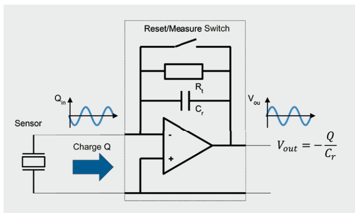
Circuit diagram of a charge amplifier
