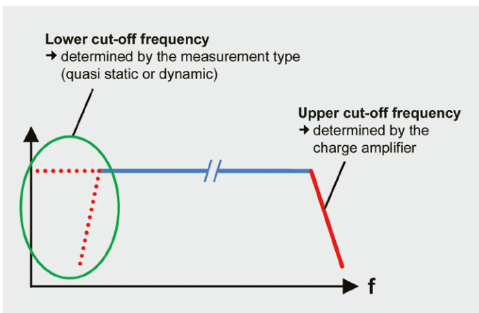
Frequency range: charge amplifier
