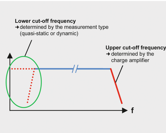
Frequency range: charge amplifier
