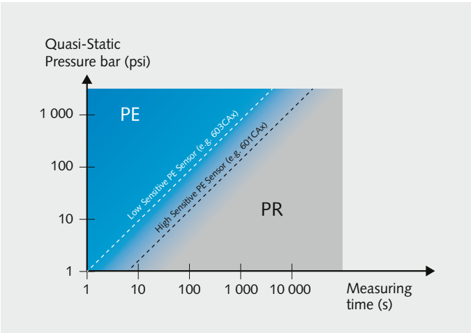
Measuring times and pressure ranges: piezoelectric (PE) vs. piezoresistive (PR) (basis: drift ±0.05 pC/s and measurement error of 1%)
