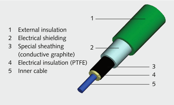
Structure of a Kistler high-impedance cable
