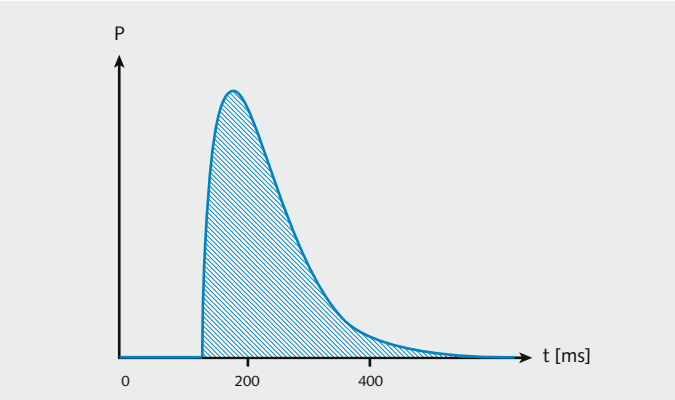
Measurement of fast pressure rise times
