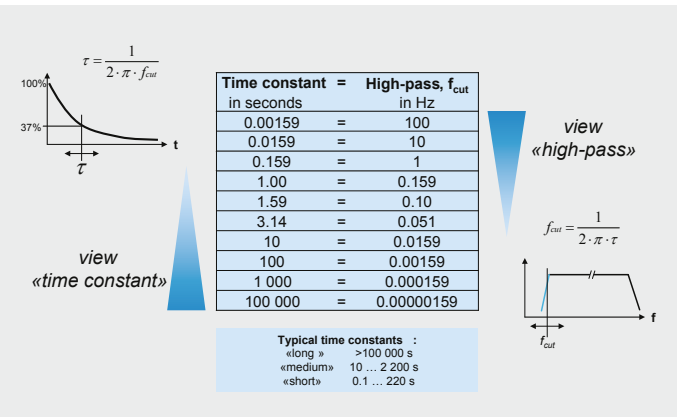
Time constant vs. high pass
