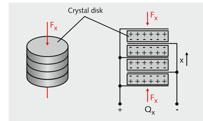
Possibility of increasing the charge yielded
