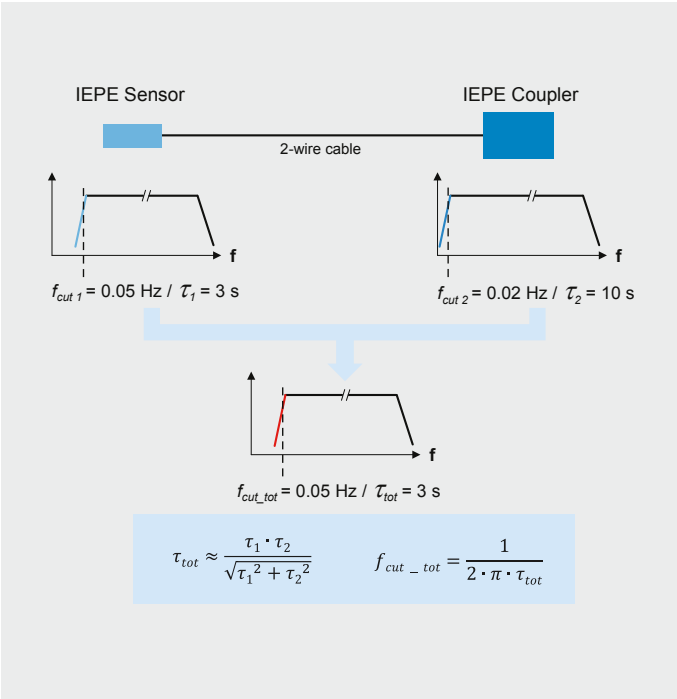
IEPE measuring chain – time constant and cut-off frequency
