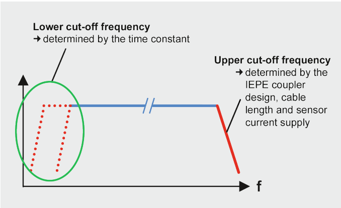
Frequency range IEPE coupler
