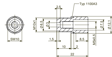
Fig. 12. Engine adapter M10 Type 6595A1Q01
