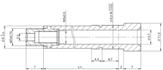
Fig. 2. Mounting sleeve M7 Type 6595ASP...
