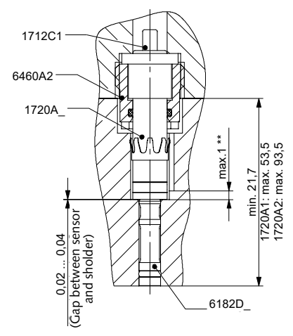
Fig. 12: Installation Type 6182D...UNR... resp. Type 6182D_ULR_ with charge conducting spacer sleeve
