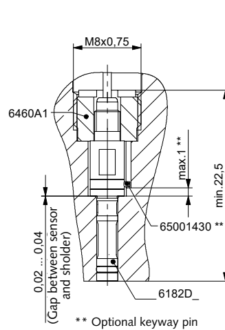
Fig. 11: Installation Type 6182D...UMR... with mounting nut
