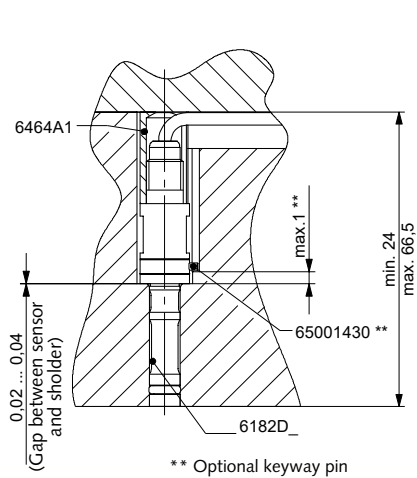
Fig. 10: Installation Type 6182D...USR... with spacer sleeve
