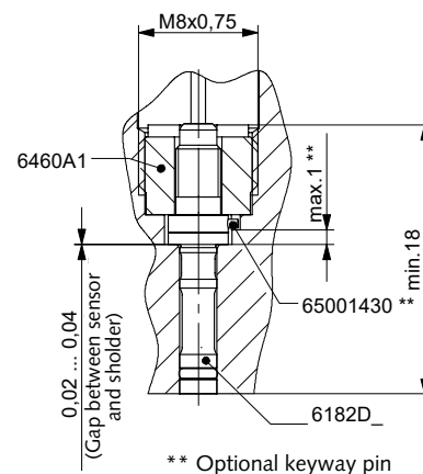
Fig. 14: Installation of Type 6182DXUSRS... or 6182DYUSRS... with mounting nut
