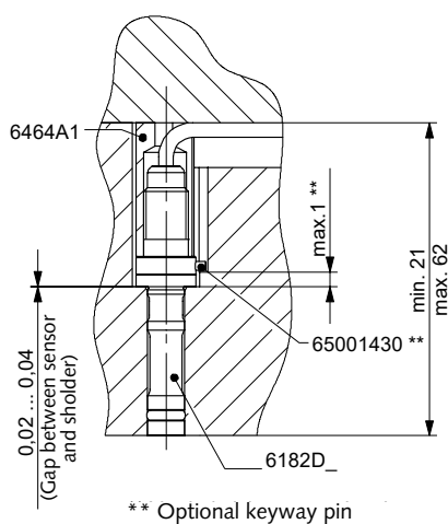
Figure 13: Installation of Type 6182DXUSRS... or 6182DYUSRS... with spacer sleeve
