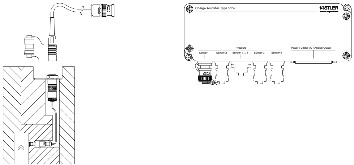
Fig. 1: Sensor Type 6182D with charge amplifier Type 5159A
