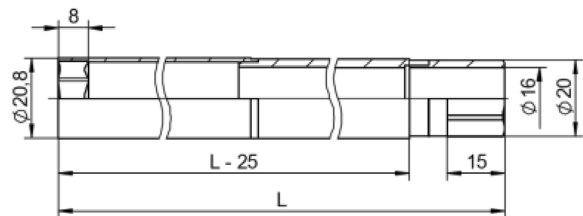
Fig. 7: Mounting wrench Type 1300A4SP100-400
