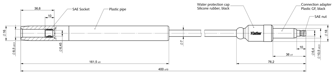
Fig. 8: Ignition extension cable for SAE connection Type 1500B97A1/1500B97A2
