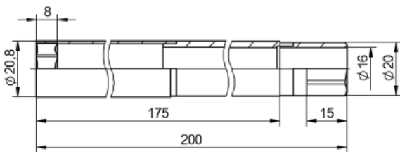
Fig. 6: Mounting wrench Type 1300A4
