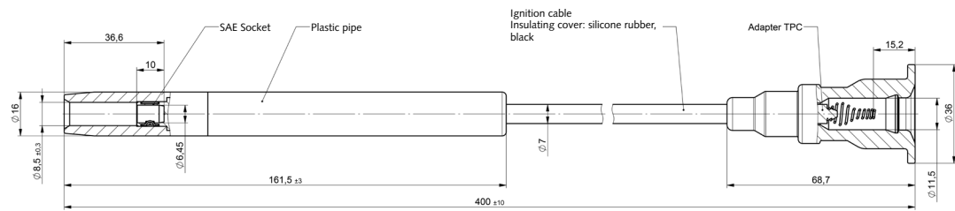
Fig. 9: Ignition extension cable for SAE connection with TPC Adapter Type 1500B97A3/1500B97A4
