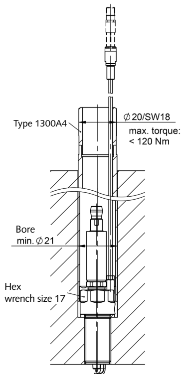
Fig. 1: Installation with a bore diameter \geq 21 mm with mounting wrench Type 1300A4
