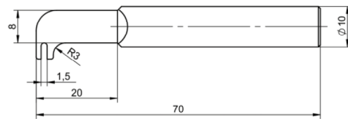
Fig. 5: Electrode spacing adjustment tool Type 1253A
