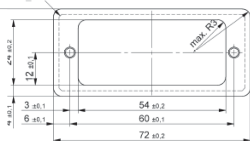
Outline of 1722A8_B
