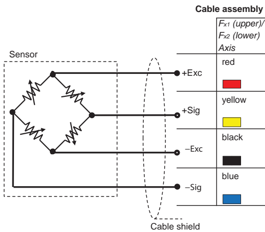
Fig. 2: Cable assembly
