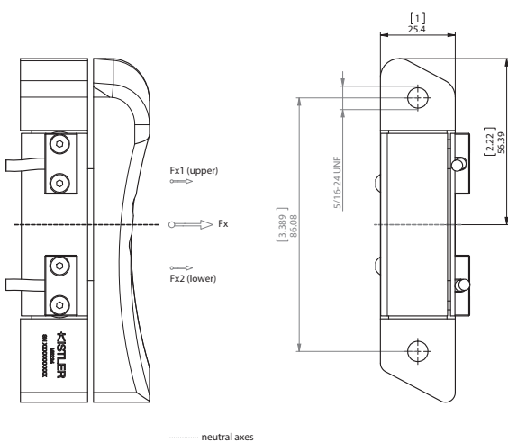
Fig. 3: Dimensions in mm (here: left side, Type M52242A...)
