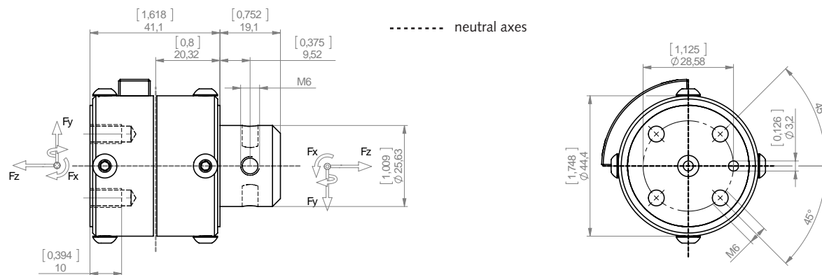
Fig. 3: Dimensions in mm
