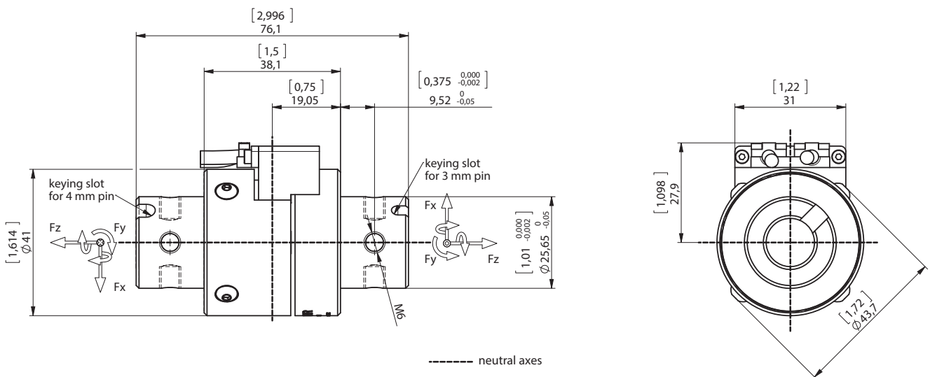
Fig. 3: Dimensions in mm and direction of action
