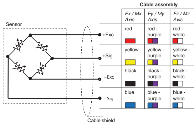
Fig. 2: Cable assembly
