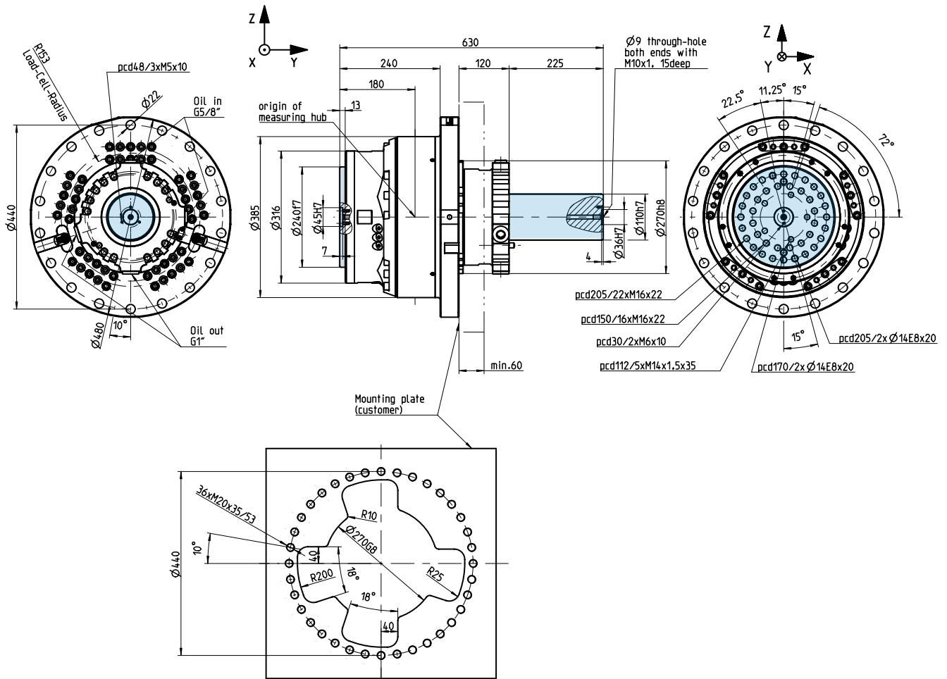
Fig. 1: Assembly drawing RoaDyn S5MT; rotating parts are highlighted in blue
