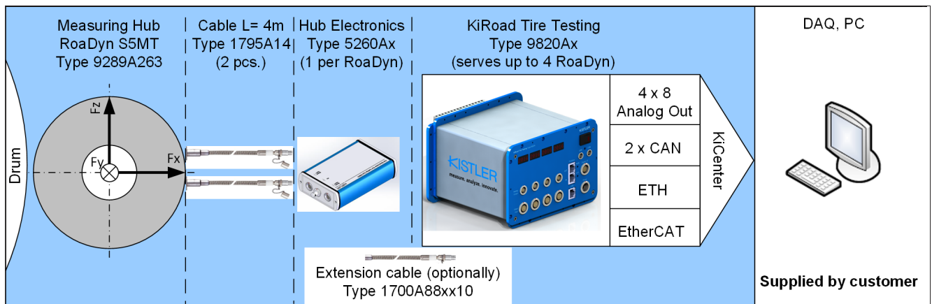
Fig. 3: Digital measuring chain RoaDyn S5MT
