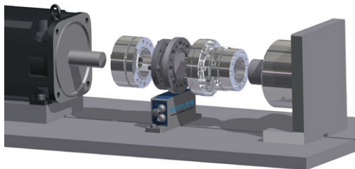
Adapter Flange + Coupling Type 2305A... Variant S: Tension Ring Hube
