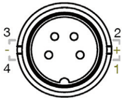
Abb. 9: M12, 4-polig, male
