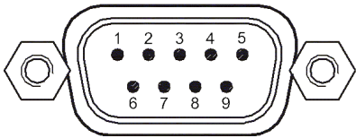
Abb. 7: 9-polig, male
