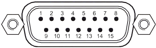
Abb. 6: 15-polig, male
