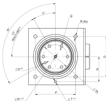
Fig. 1: Dimensions NC joining module NCFN Type 2153A...
