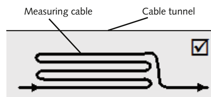
To reduce the inductive areas it's recommended to laying the measuring sensor cable in bifilar form
