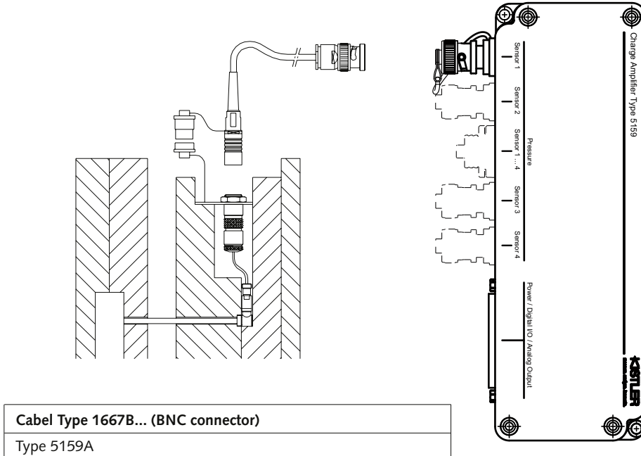
Fig. 4: Sensor Type 9204B... with charge amplifier Type 5159A
